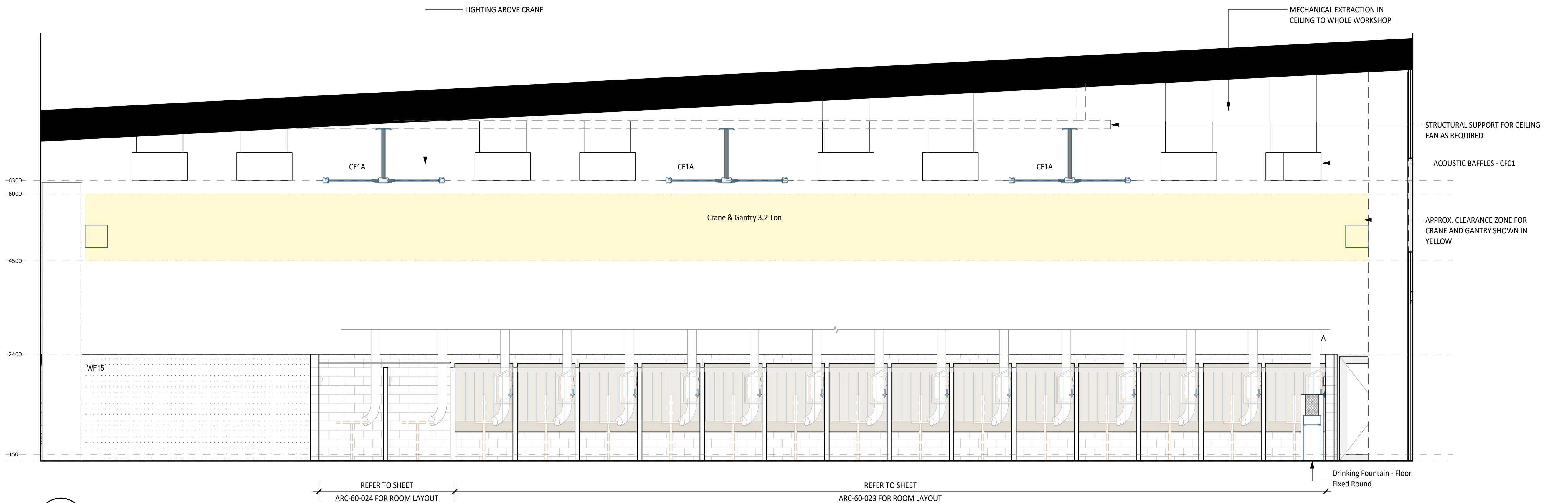
2 60-020 ELEVATION DETAIL 1 : 50
